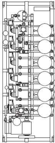
Choke and Kill Manifold
